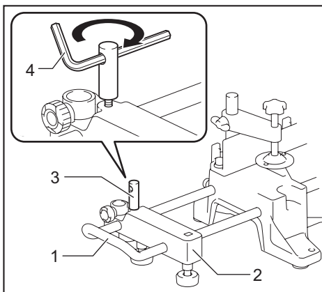
► 1. Holder 2. Holder assembly 3. Fence shaft 4. Hex wrench
