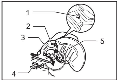
▶ 1. Shaft lock 2. Arrow 3. Blade case 4. Hex wrench 5. Hex socket bolt
