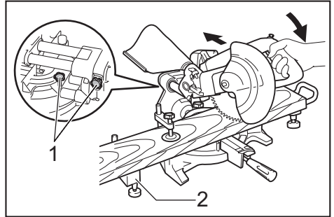
► 1. Thumb screw 2. Holder assembly
