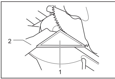
► 1. Triangular rule 2. Guide fence
